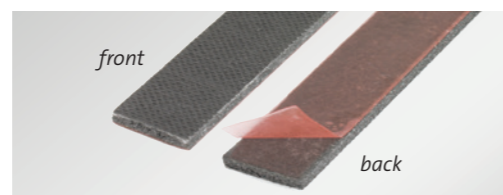
Also available: IFPS fire penetration seal stripe, 900 x 17 x 2.7 mm, self-adhesive Order No. 99303
