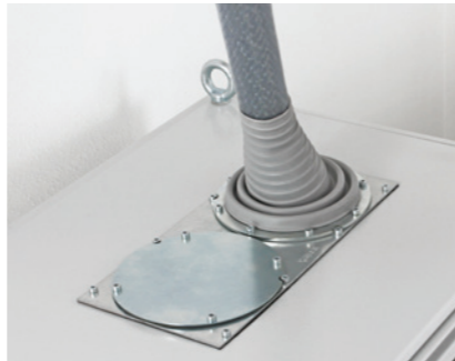
Routing of a rigid supply line through a closed enclosure roof via module plates. Cut-out size 314 × 144 mm.
