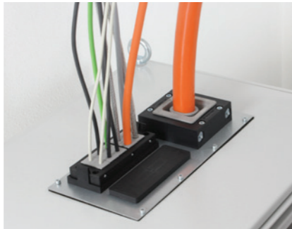
Routing of several cables with and without connectors through a closed enclosure roof via module plates. Cut-out size 314 × 144 mm.
