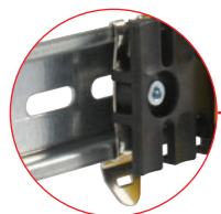
Wide mounting type variety: top hat DIN rail/C-rail snap mount, screw mount
