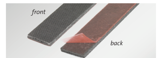
Also available: IFPS fire penetration seal stripe, 900 x 17 x 2.7 mm, self-adhesive Order No. 99303
