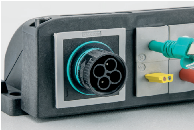
The cable entry frames enable the integration of the IMAS-CONNECT™ adapter grommets
