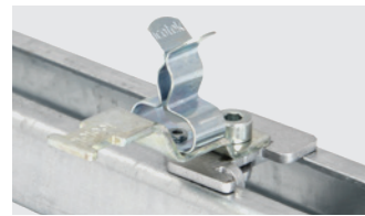
Assembly on 30 mm C-rails
