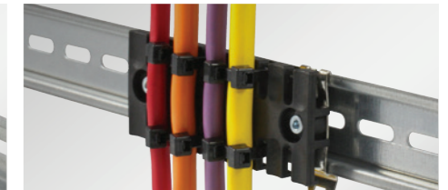
Strain relief plates for 35 mm top hat DIN rail snap mount
