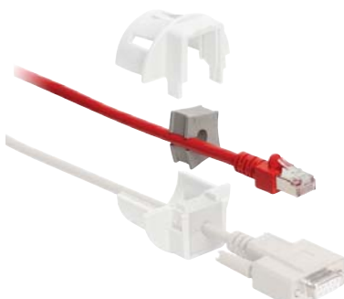
QT grommet in combination with QVT-CLICK
