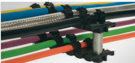
Spacers for multilayer mounting of strain relief plates
